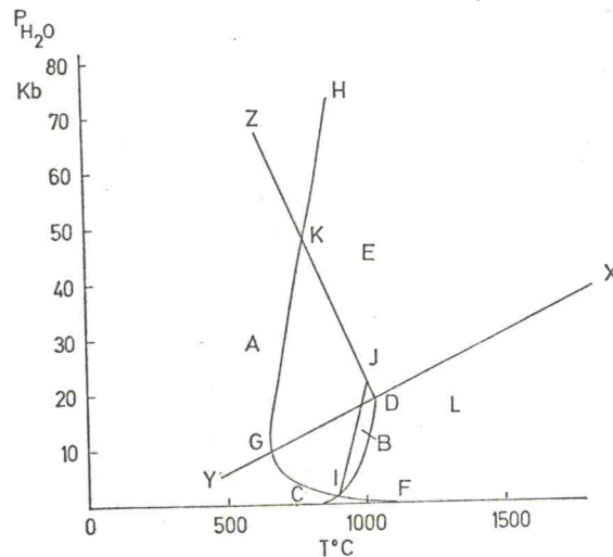
Fig. 3. An approximate diagram showing the region of stability of eclogites (region bounded by Z-K-H ) in a system with excess water. For further details see text
